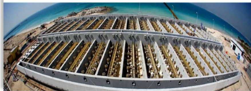
Dubai - The World's Largest DynaSand Plant - 7000 LPS
